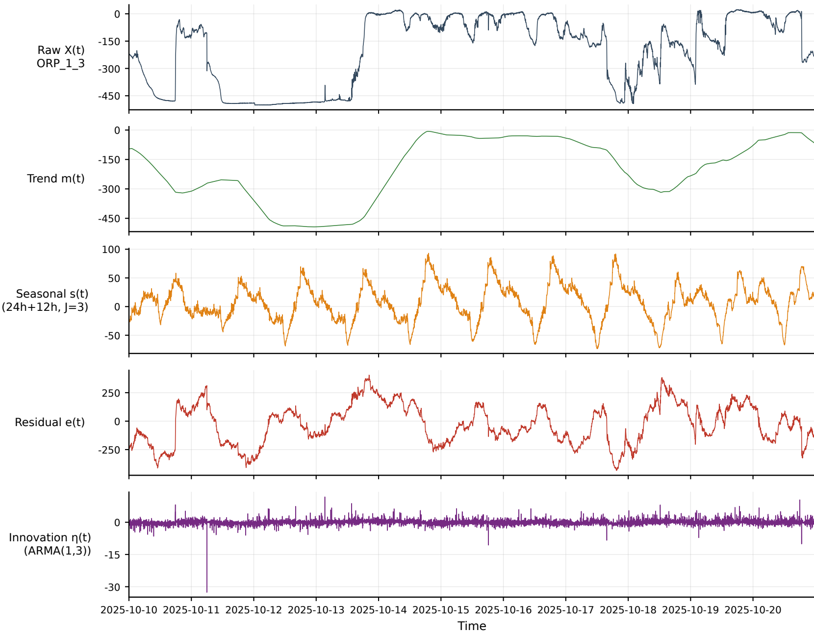
Multi-scale decomposition — ORP_1_3 (pre_anoxic_rear, min) [2025-10-10~2025-10-20]
